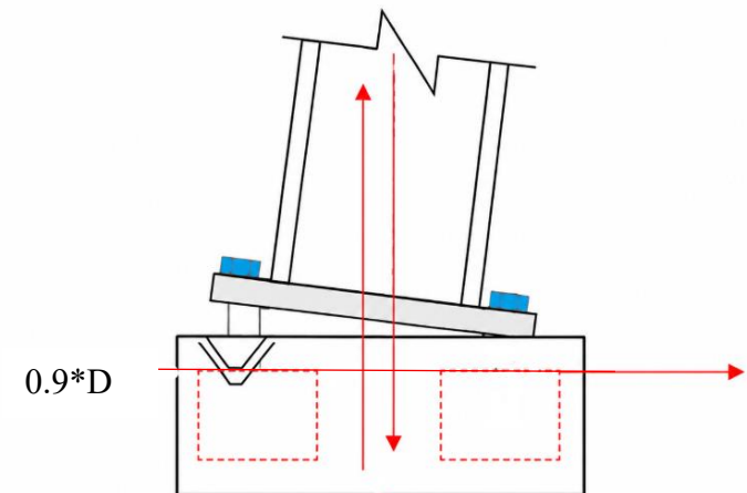
Anchor bolt failure (tension side)
